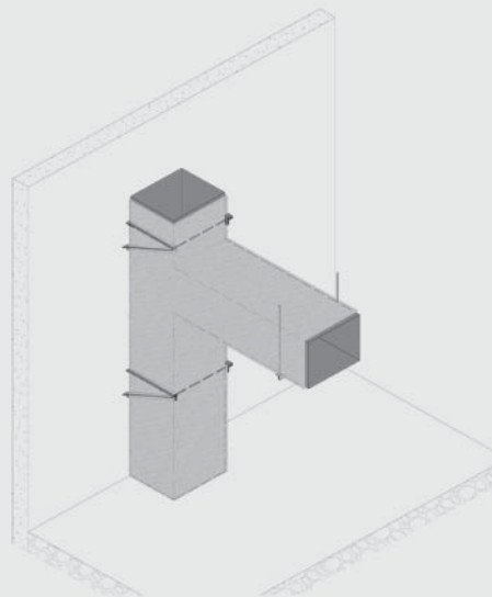
5. Vertical anchor and horizontal couplingl.
